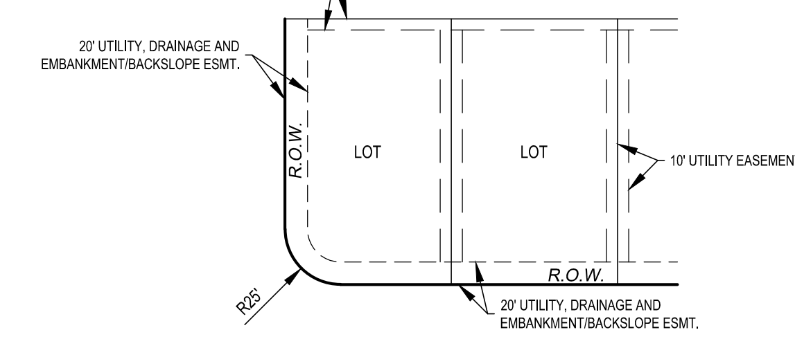
TYPICAL TRACT LAYOUT NOT-TO-SCALE
